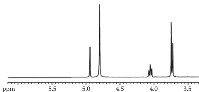
FIGURE 12.2 ^1\text{H} NMR spectrum (300 MHz) in \text{D}_2\text{O} of vitamin C.
