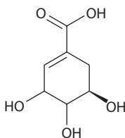
FIGURE 4.8 Structure of shikimic acid.
