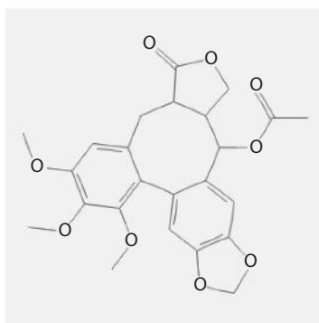
FIGURE 6.13 Other lignan structures represented by podophyllotoxin and steganacin.
