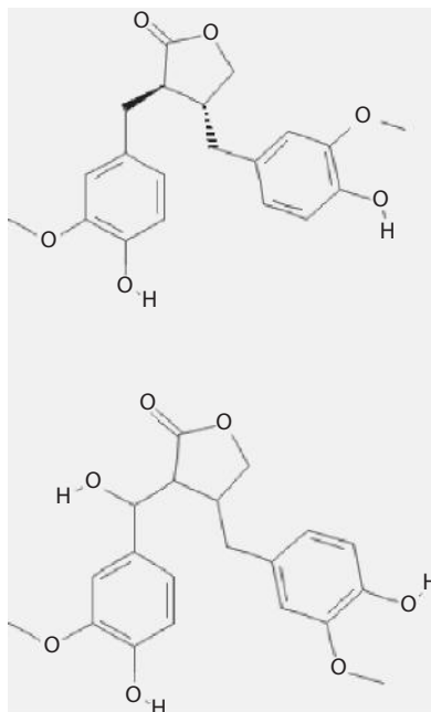
FIGURE 6.14 Structures of the lignans, matairesinol, and 7-hydroxmatairesinol.
