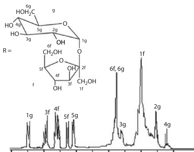
FIGURE 5.4 Chemical structure and 1 H NMR spectrum of sucrose with chemical assignments.
