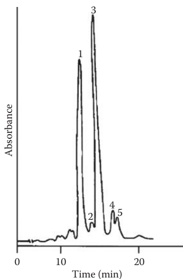
FIGURE 11.5 HPLC separation of carotenoids in carrots.
