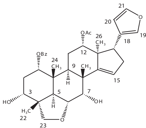
FIGURE 10.11 Example of naturally occurring limonoids from plants in Papua New Guinea.
