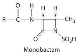
FIGURE 9.7 The core monobactam chemical structure, R represents various amino acid side chains.
